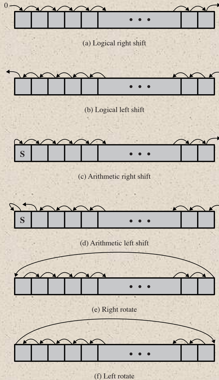
Figure 12.6 Shift and Rotate Operations
